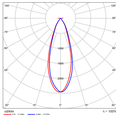
Polar LDC
